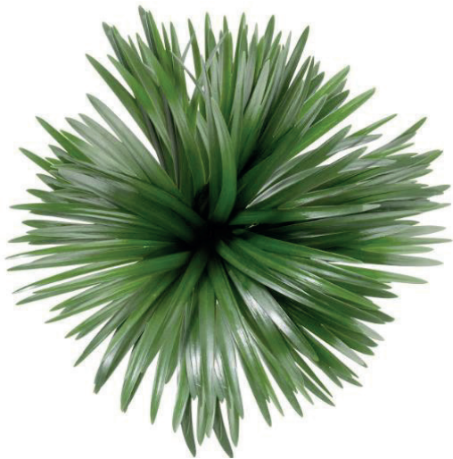
Lily Grass
